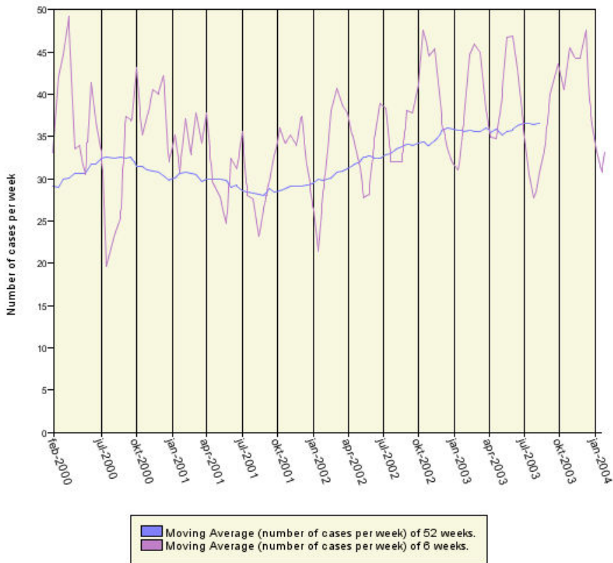
Hepatitis B - Trend
