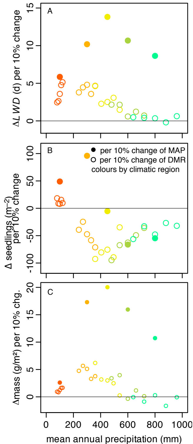
Fig. A4.1. Changes of variables expressed per 10% change of MAP (slope of black lines of Fig. 2 A, C, E) [dots, ●] and, for comparison, changes of variables per 10% change of DMR (slope of thin coloured lines of Fig. 2 B, D, F) [circles, ○]. This shows the effect of the relative change of DMR and MAP as expected for the cited climate change scenarios. Colours correspond to different climatic regions (red: arid, orange: semiarid, yellow: dry Mediterranean, green: typical Mediterranean, bluegreen: mesic Mediterranean).
