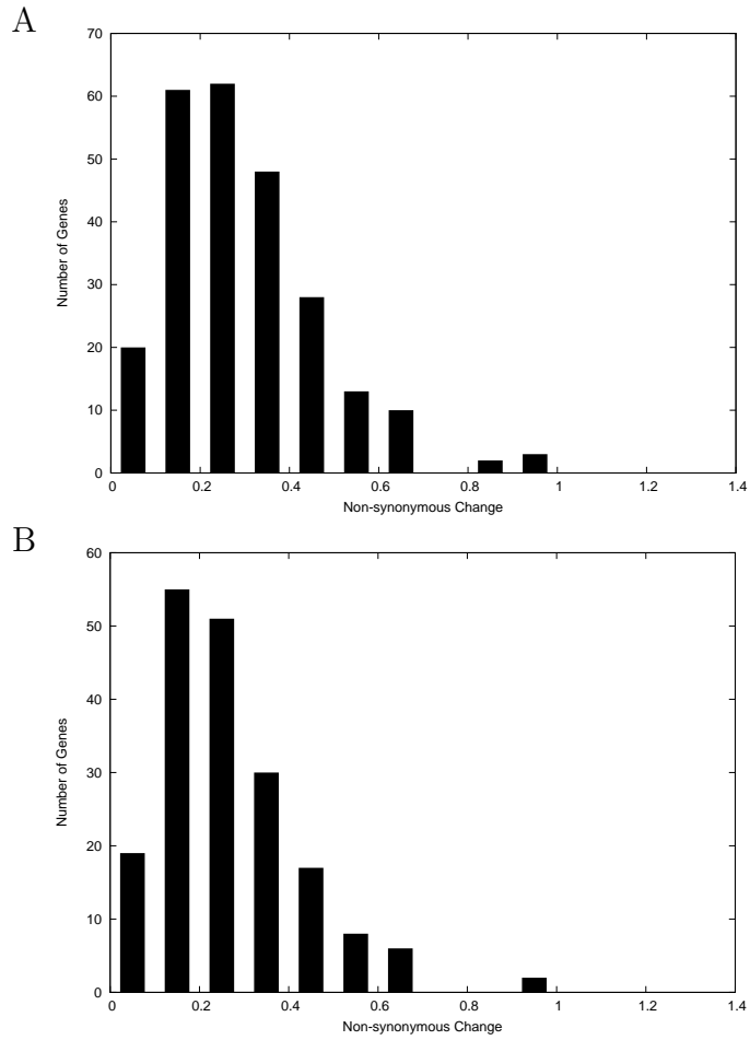
Figure S.1: Non-synonymous change of the genes present in Cgl and Cef. A, genes present in Cgl and Cef; B, genes present in Cgl and Cef and having matches in the database. Genes show similar rates of evolution by only looking at the genes having matches elsewhere the genome database.
