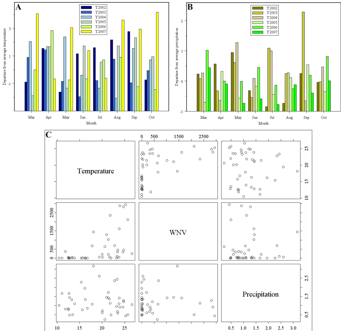
Figure 4 Departure from average temperature and precipitation in Indianapolis in 2002–2007 from March to October. Figure 4A shows the departure from average temperature in Indianapolis. Units: °C. Figure 4B presents the departure from average precipitation in Indianapolis. Units: meters. Figure 4C shows the relationships between temperature, precipitation, and WNV dissemination.
