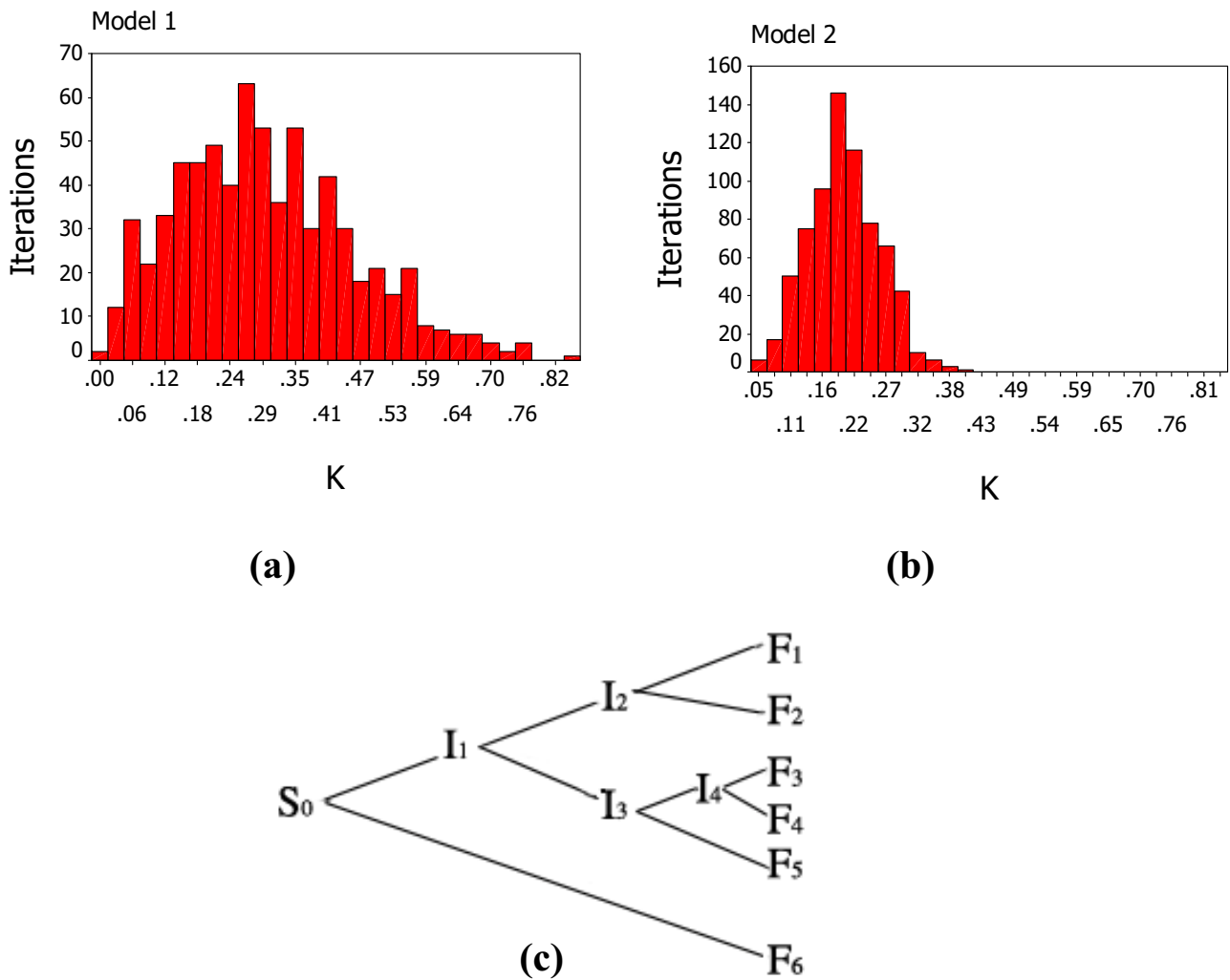
Figure 3 Estimated K for Monte Carlo Simulation The distribution of estimated K is shown in a) and b): a) Model I; b) Model 2. The common phylogenetic tree is shown in c)
