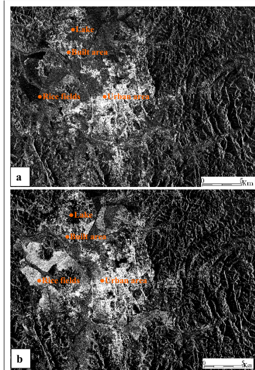
Figure 3 ASAR_IMP_1P images illustrating changes between January and July 2004. Difference between images acquired in January and July 2004.
