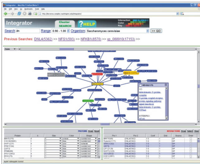
Figure 2 The Integrator network viewer interface. Shown here is a representative network search result around a selected node (yellow) with various other nodes modified for color, size, or shape. The center frame contains the main interactive graph viewer. Users can traverse a network by clicking on nodes. Double-clicking on a node opens a window containing detailed sequence and annotation information. Hovering over nodes also brings up tool tips containing GO and Interpro annotations. Hovering over edges shows tool tips with edge confidence data. Right-click contextual menus also exist for nodes and edges which allow for search, hiding, showing, and changing their visual properties. The slider bar at the top of the graph viewer modulates zoom, rotation, or viewable neighborhood size. Below this are two interactive network tables, nodes on the left, edges on the right. These tables can be used to sort and modify various node and edge properties in the viewer.
