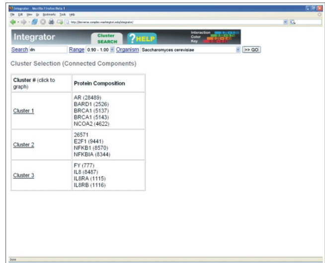
Figure 3 Multiple protein identifier search results. A representative search result where three clusters (defined by connected graph components) are shown with their constituent nodes. Each of the individual clusters can be viewed graphically by following their hyperlinks.
