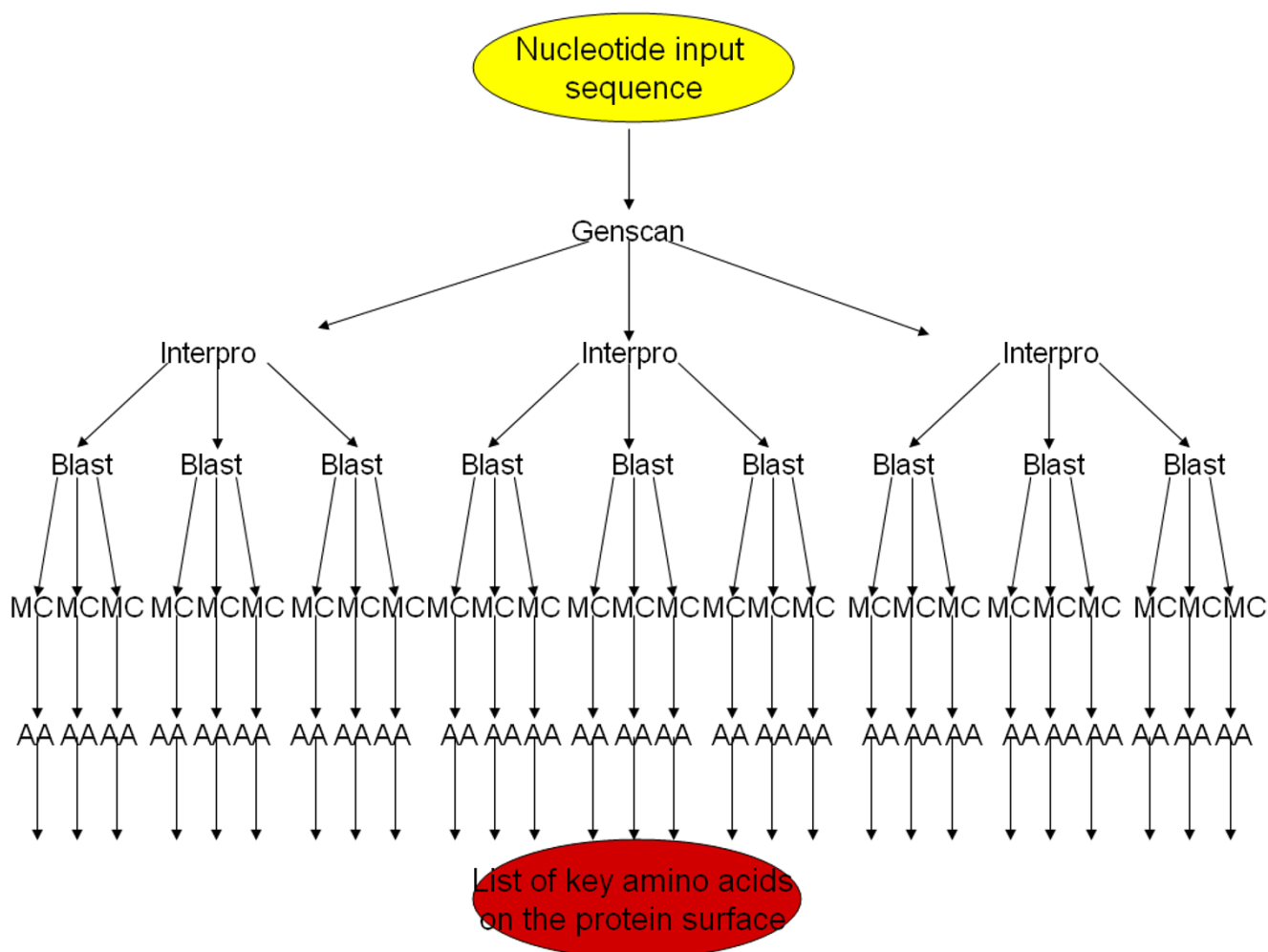
Figure 2 In the first three analysis steps the computation tends to expand, but the information collapse in the definition of few key amino acids.
