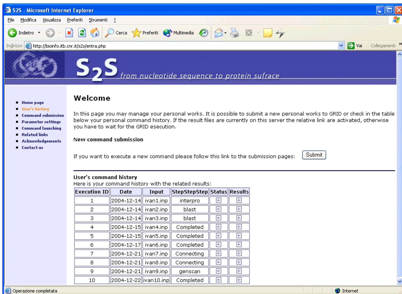
Figure 5 The personal home page of a user after the log in procedure. From this page each user can control the state of advancement of the workflows submitted to the grid platform.
