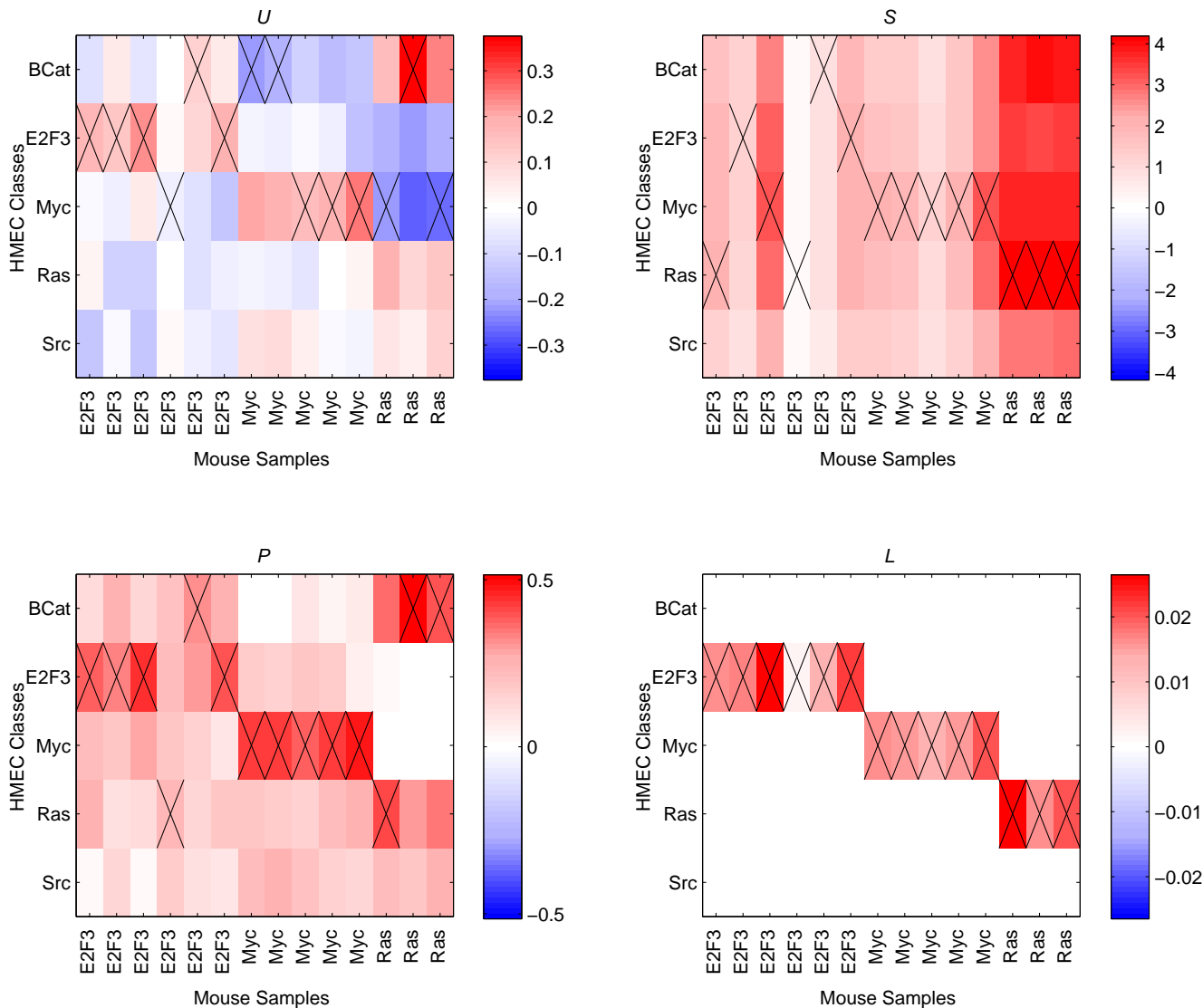
Figure 3 Results on HMEC-Mouse data. Heatmaps showing the w vectors for the decomposition of the mouse samples into the HMEC classes. The four heatmaps correspond to the four decomposition variants, U , P , S , and L , as indicated above each of the heatmaps. Each heatmap lists the 14 mouse samples along the x-axis, and the five HMEC classes along the y-axis. The heatmap reflects the w vectors that were obtained by decomposing each mouse sample separately. Each column contains one cross, indicating the largest absolute weight in that particular w vector, and thus the class assignment for that particular mouse sample. These solutions correspond to the case where the union of top 70 most differentiating genes for the separate one-versus-rest HMEC class comparisons are employed to represent the HMEC classes.
