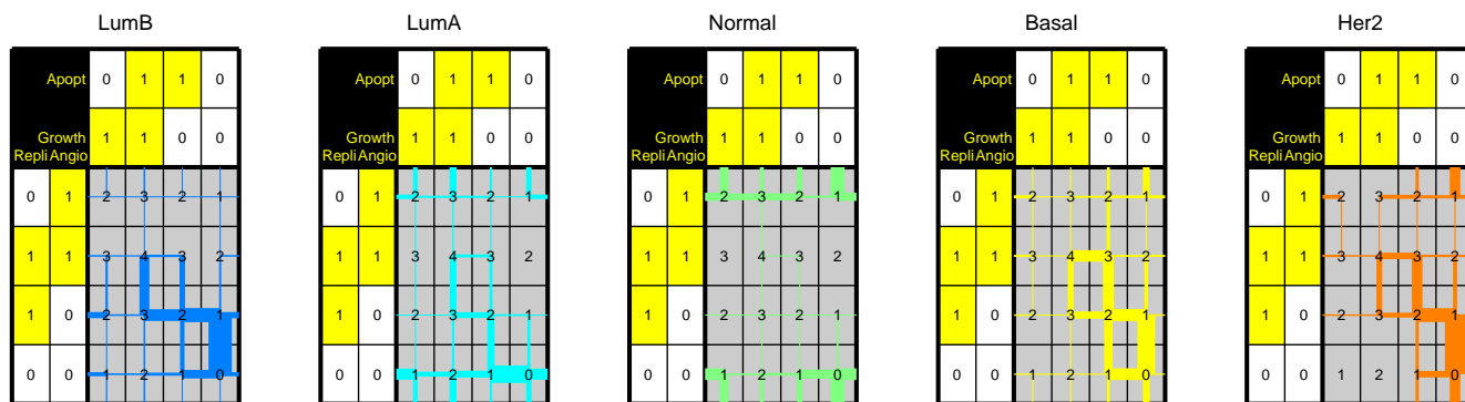
Figure 9 Visualization of Lasso shrinkage in the Hu subtypes. Table indicating the order in which the weights in w become non-zero, when changing \lambda . The figure shows the results for the human samples split over the five subgroups defined by Hu et al. [2]. Gene sets that correspond to these four Hanahan hallmarks were chosen as components. The linewidth is proportional to the total number of samples in that clinical subgroup. Apopt: Apoptosis; Growth: Growth; Angio: Angiogenesis; Repli: DNA Replication.
