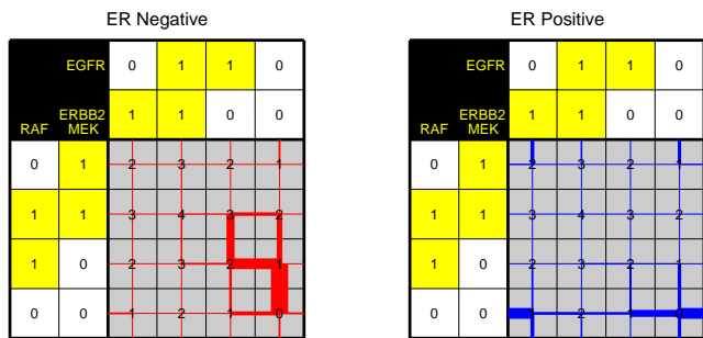
Figure 8 Visualization of Lasso shrinkage in the ER subgroups. Table indicating the order in which the weights in w become non-zero, when changing \lambda . The figure shows the results for the ER negative (left) and ER positive (right) groups separately. The linewidth is proportional to the total number of samples in the ER negative/positive subgroup, respectively.
