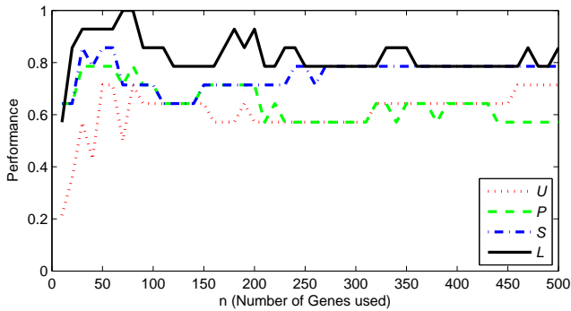
Figure 4 Performance on the HMEC-Mouse data. Performance (y-axis) of the four decomposition variants ( U , P , S , and L ), for a range of the selected number of genes n (along the x-axis). The performance indicates the fraction of mouse samples for which the largest absolute weight in w corresponds to the correct HMEC class. The number of genes, n , was varied from 10 to 500 in steps of 10.
