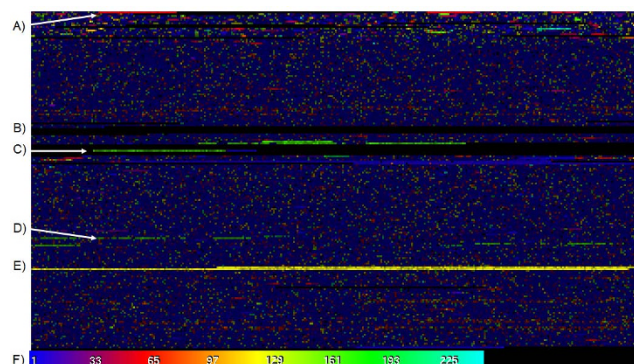
Figure 2 Repeat Overview of Human Y Chromosome. This visualization of the first half of the Y chromosome is colored according to the best local alignment score. Chromosome Y was selected for the diversity of repeats. The second half of the Y chromosome has only a very small section near the end that has been sequenced so it is not included in this view. A) The bright red streak is the same 61-mer repeat seen in Figure 1B. B) The pure black streaks are regions of unsequenced N's. C) The green areas in the middle are 171-mer alpha satellite near the centromeres. D) A second region of alpha satellite repeat (with lower percent similarity) separated from the centromere starting around nucleotide #18,293,073 (March 2006 assembly). This is actually part of a large scale palindrome where the reverse complement of the alpha satellite starts at # 18,822,065. E) The bright yellow region is a very large, 125-mer tandem repeat that comprises a quarter million nucleotides. F) Colors correspond to the frequency spectrum ranging from 1 - 250 nucleotide offsets. Brightness is based on the degree of local self-similarity, with brighter colors corresponding to better self-similarity.
