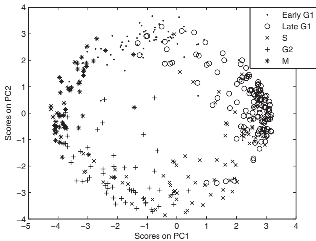
Figure 6 Scores plot of Yeast cell-cycle dataset. The first two PCs capture 65% variance.
